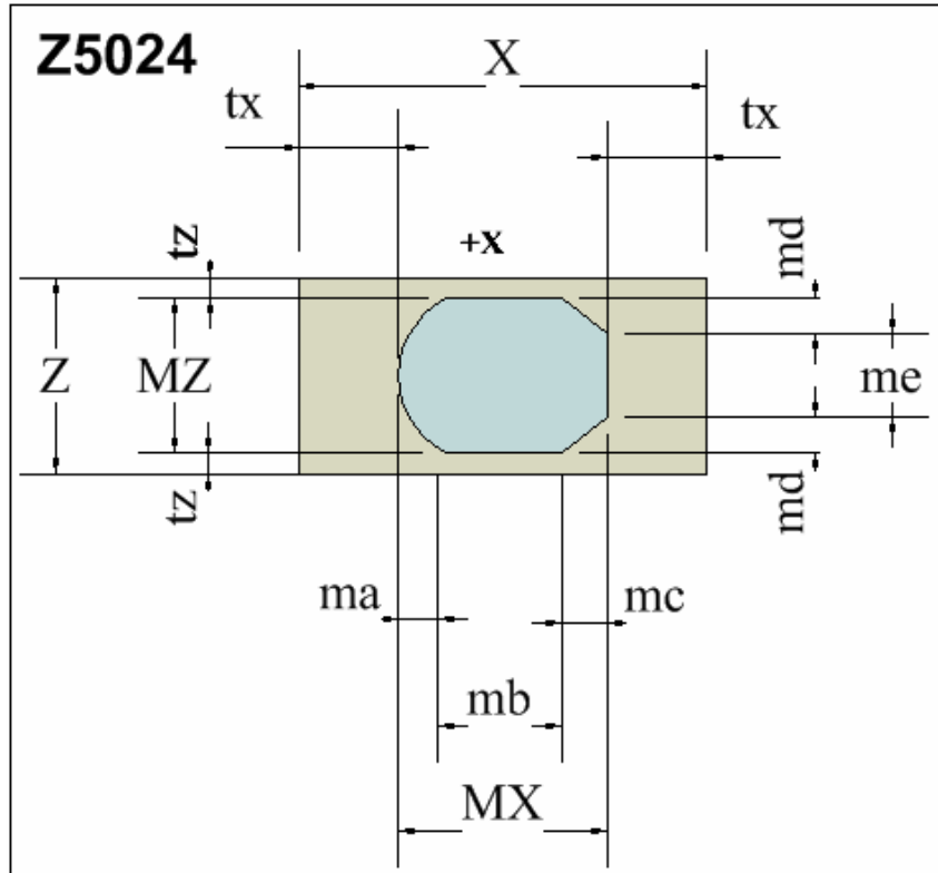
Z5024 Blank drawing and dimensions
