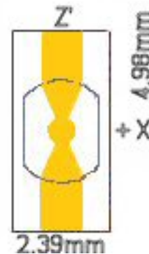
Typical electrode pattern for UM-1 mount
